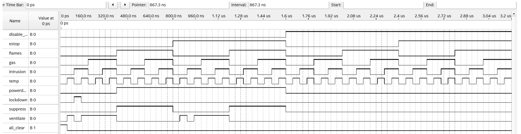
Figure 3. Waveform utilizing decreasing binary periods to test all conditions of the safety-logic module
