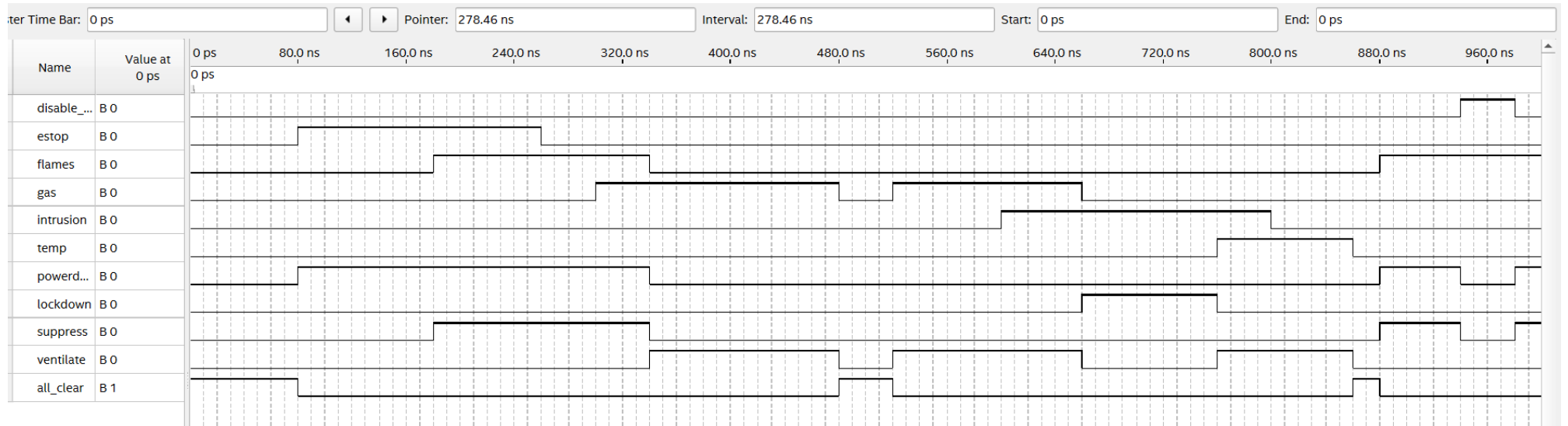
Figure 2. Waveform testing several conditions of the safety-logic module with their corresponding outputs.
