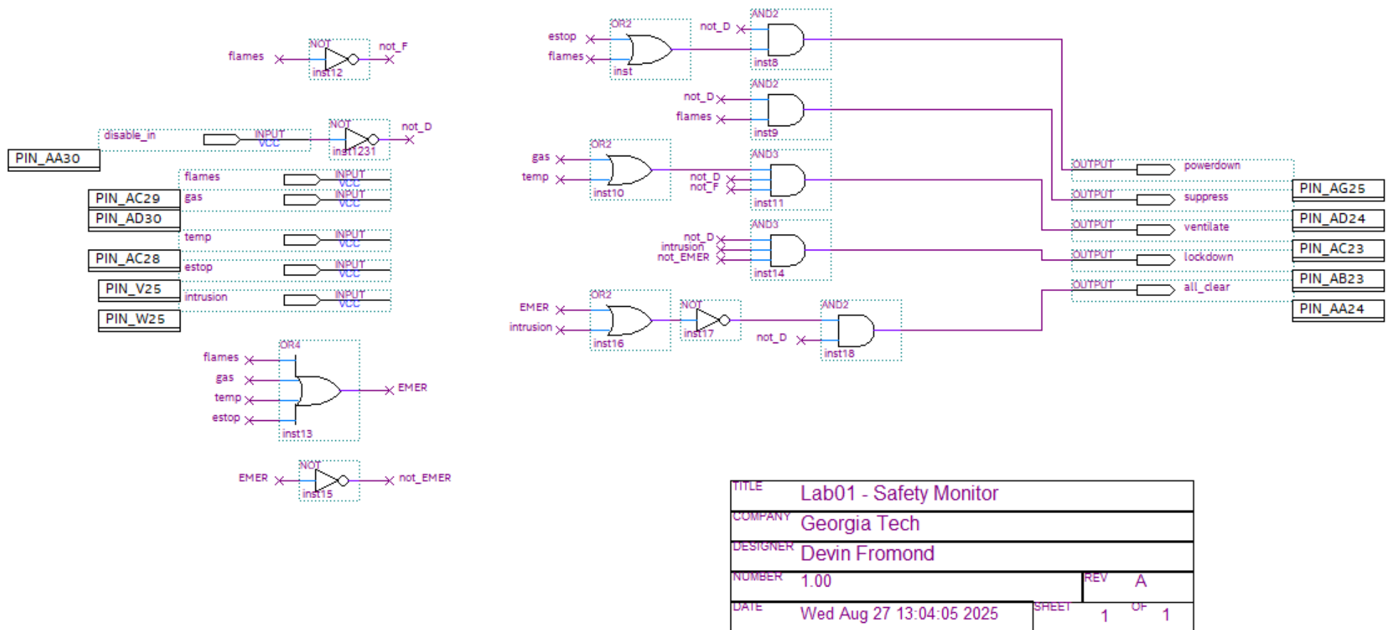
Figure 4. Schematic containing pins for an FPGA with designation 5CSXFC6D6F31C6 (identical logic to Figure 1.).
