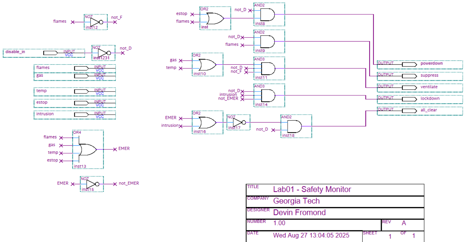
Figure 1. Schematic for the logical expressions pertaining to a safety-logic module with the outputs of powerdown ( /D \cdot (E + F) ), suppress ( /D \cdot F ), ventilate ( /D \cdot F \cdot (G + T) ), lockdown ( /D \cdot I \cdot EMER ), and all_clear ( /D \cdot /(EMER + I) ), where EMER = F + G + T + E and the state abbreviations are the first letter of the state as pictured on the left of the diagram.
